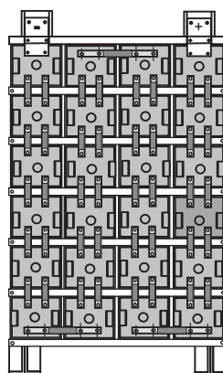
Front View 24 cells 2TLGM750 to 1500 4 post cells
