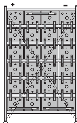
Front view 24 cells 2TLGM750 to 1500 4 post cells
