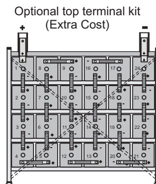
Front view 24 cells 2TLGM100 to 700 2 post cells
