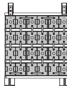
Front View 24 cells 2TLGM100 to 700 2 post cells
