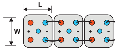
BATTERY TYPE 2ETG 700 to 1500
