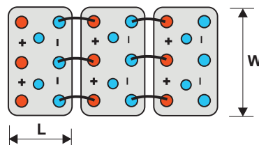
BATTERY TYPE 2ETG 1750 to 2000
