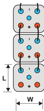
TYPE 2ETG 700 to 1500
