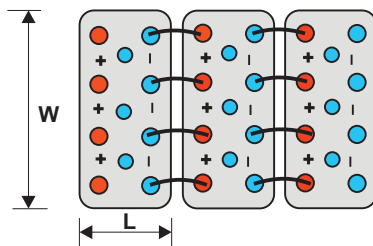
BATTERY TYPE 2ETG 2500 & 3000
