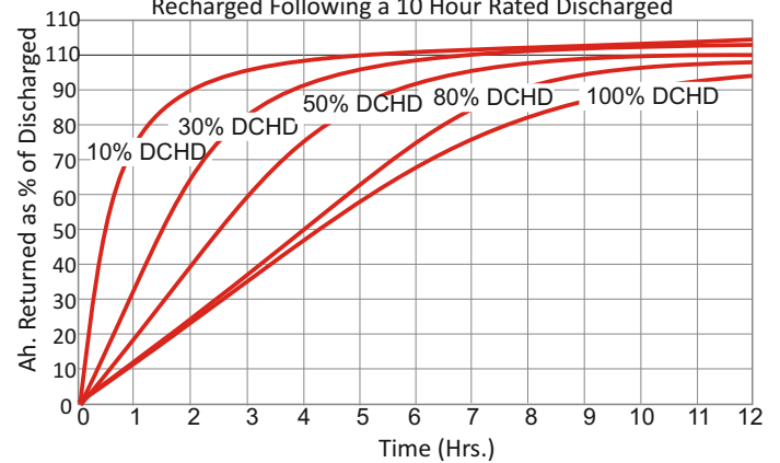
Recharge Profile @ 2.27Vpc & C/10 Amps Recharged Following a 10 Hour Rated Discharge
